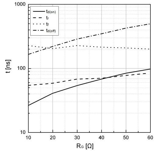
Fig 14. Typical switching times as a function of R_G ( T_{Vj}=175^\circ\text{C} )
